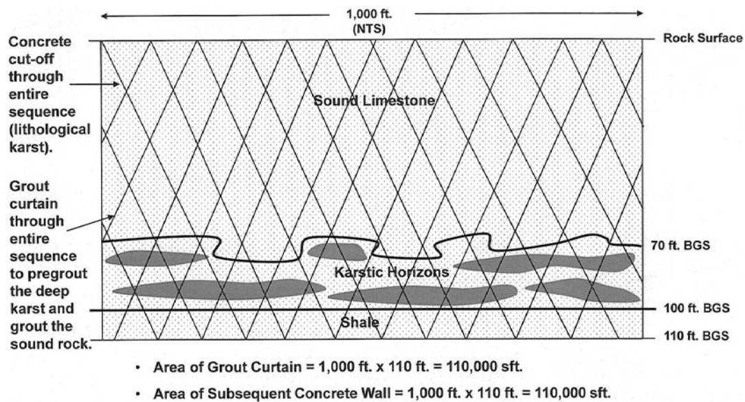
Figure 1 b). Heavily karstified horizons are found at depth. Therefore the concrete cut-off is required for the full extent. The grouting has pretreated the karstic horizons to permit safe concrete cut-off construction.
