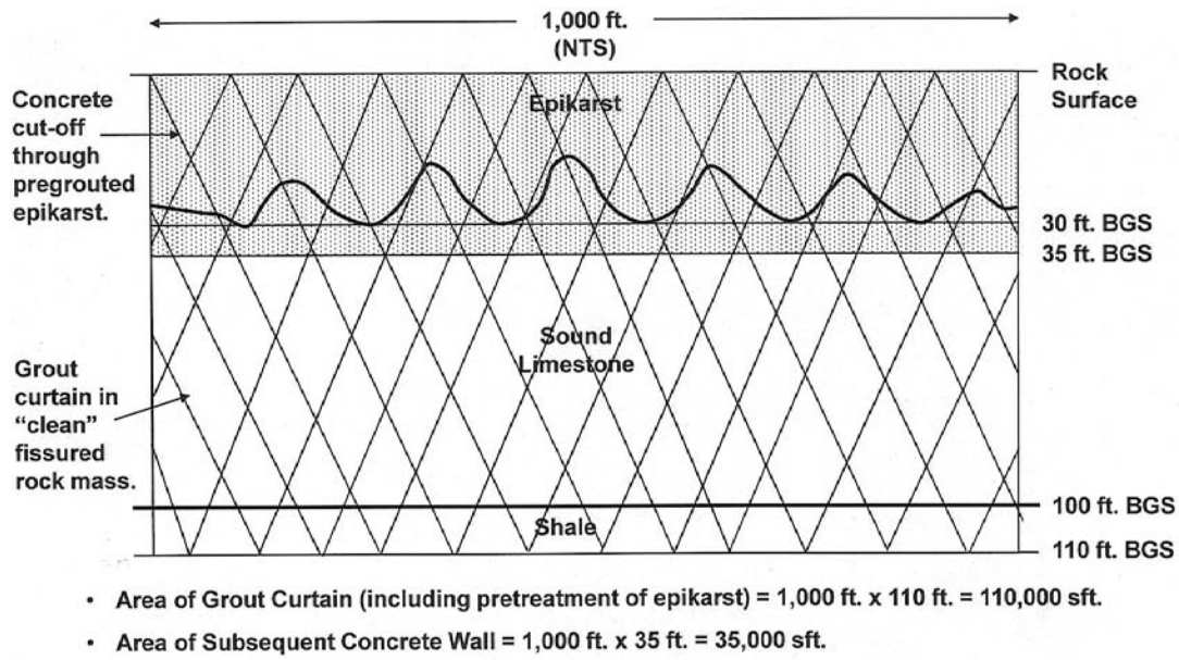
Figure 1 a). Epikarst is found during pregrouting to an average of 30 feet b.g.s. The concrete cut-off needs only to be installed to 35 feet b.g.s.
