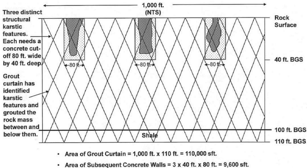
Figure 1 c). Discrete karstic features have been found, structurally driven. Thus, individual concrete cut-offs can be installed, after drilling and grouting have confirmed the extent of these features and have pretreated them to permit safe concrete cut-off construction.
