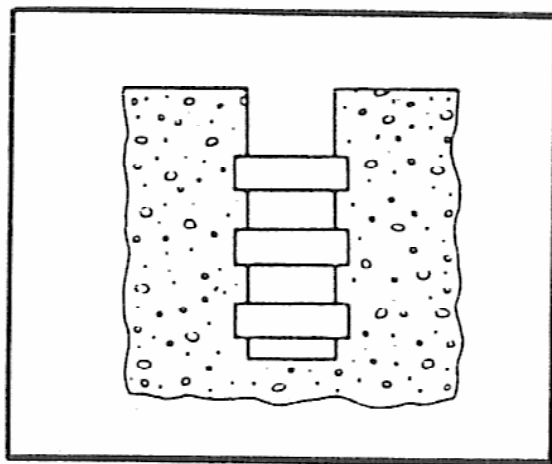
Figure 2. Typical triple-groove bonding profile produced by the Ankerbonder in a diamond cored hole. At the West Burton project, in England, two sets of triple grooves were provided per hole. (Anon, 1987)
