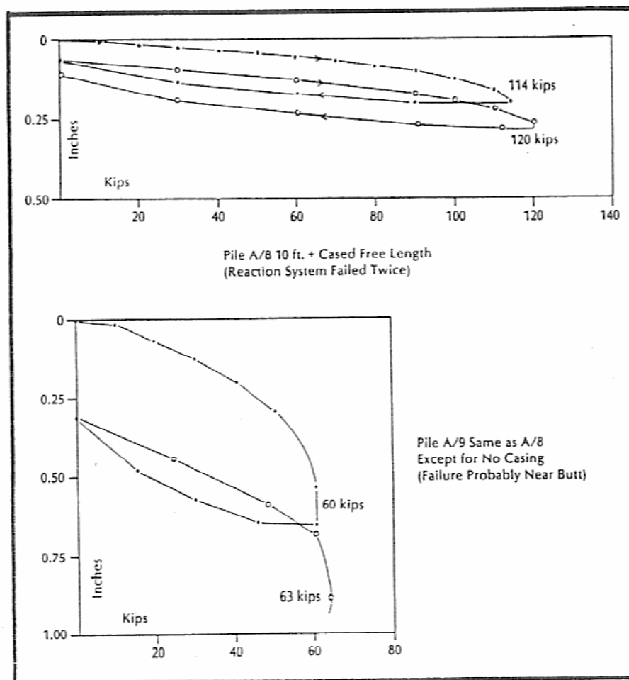
Figure 7 . Pin pile load test data from a site in Coney Island, New York, showing the benefits of a steel liner through upper strata above the bond zone. (Bruce, 1988)
